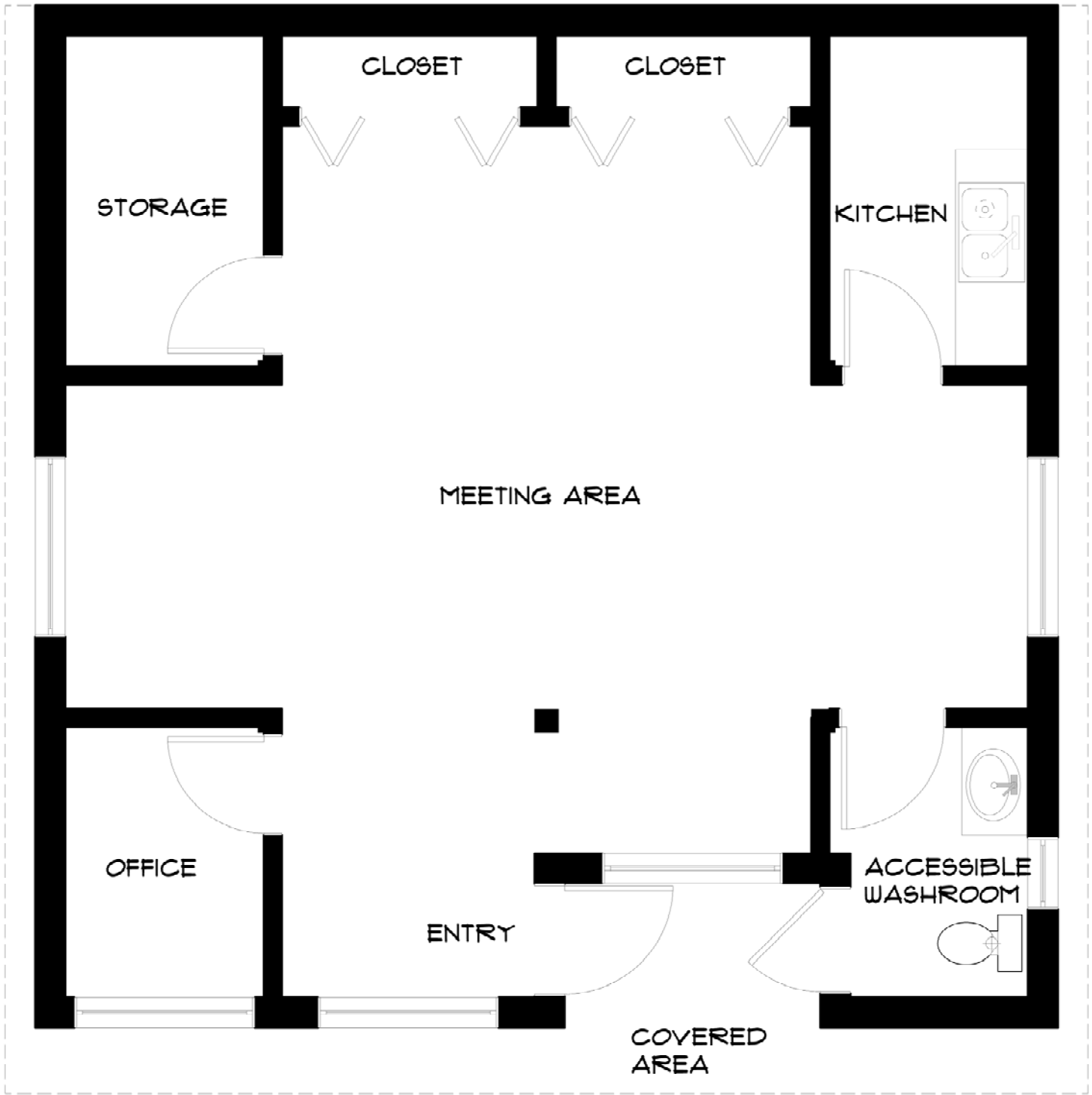
STRATHCONA PARK WILDERNESS CENTRE PARADISE MEADOWS LOWER LEVEL FLOOR PLAN 1/4" = 1' - 0"
